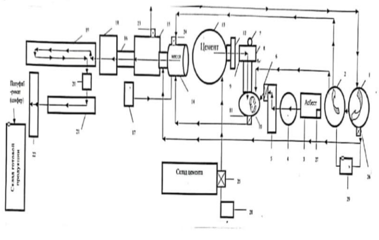
Figure-3. Layout of the line production of asbestos-containing slate
