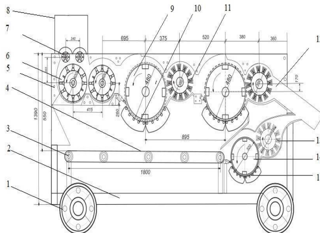
Figure 2. Schematic diagram of a cotton cleaning machine..
