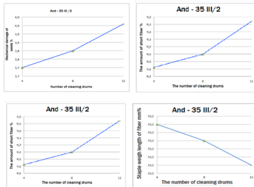
Figure 1. Mechanical damage to the seed, the amount of short fiber, the staple weight length of the fiber in mm, the mass fractions of defects and contaminants are given.
